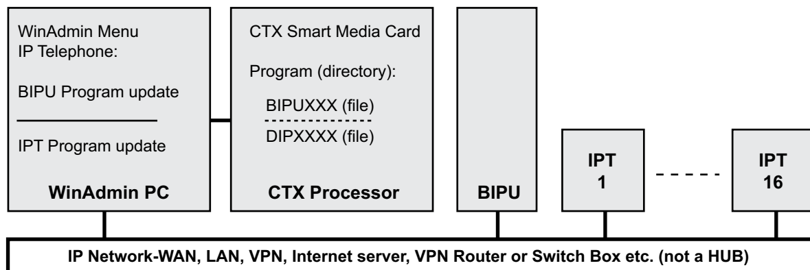
Figure E-1 FTP Server (SmartMedia card) Network Connection
