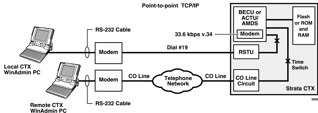
Figure 3-4 CTX WinAdmin Modem Interface Connection
