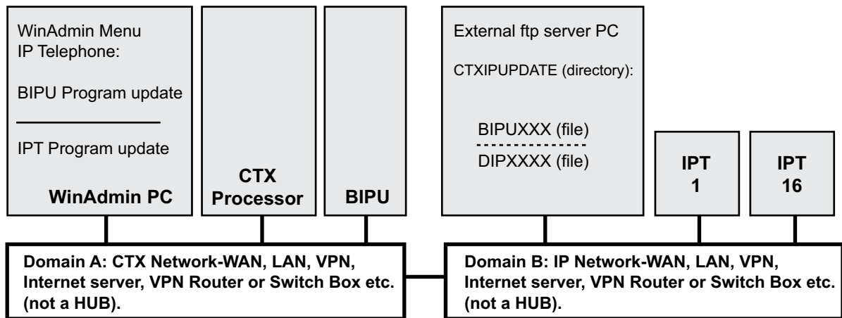
Figure E-3 FTP Server (External Server) Network Connection
