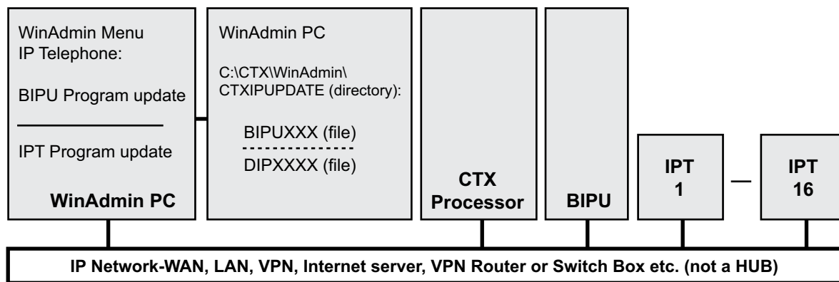
Figure E-2 FTP Server (WinAdmin PC) Network Connection
